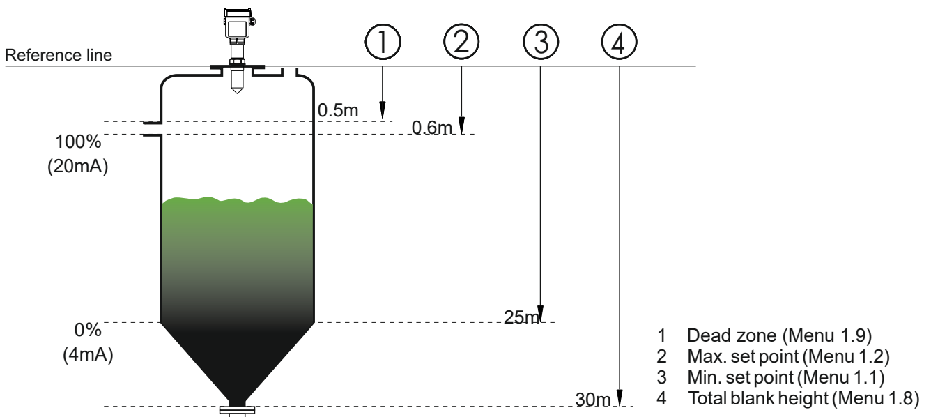
Microcom Adjustment Module
