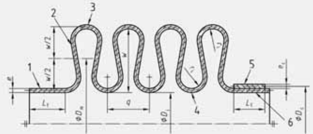
Figure 2.1 Unreinforced Bellows
