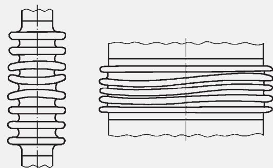
Figure 2.5 - In-Plane Squirm
